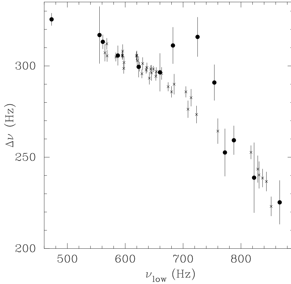
Fig. 3.— The frequency separation between the upper and the lower QPO peak as a function of the frequency of the lower QPO for 4U 1608-52 (circles). The crosses are the data obtained for Sco X-1 (van der Klis et al. 1997). The rise of \Delta\nu at \nu_{\text{low}} \sim 700 Hz in 4U 1608-52 is marginally significant.
